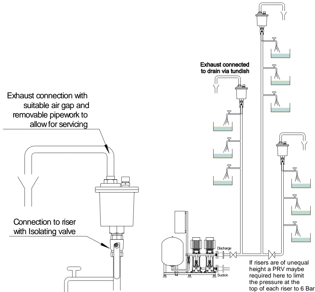
Fig. 1.1 Typical Pipework arrangement Fig. 1.2 Example of multi-riser use
